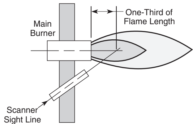
Figure 2 UV Scanner Sighting
