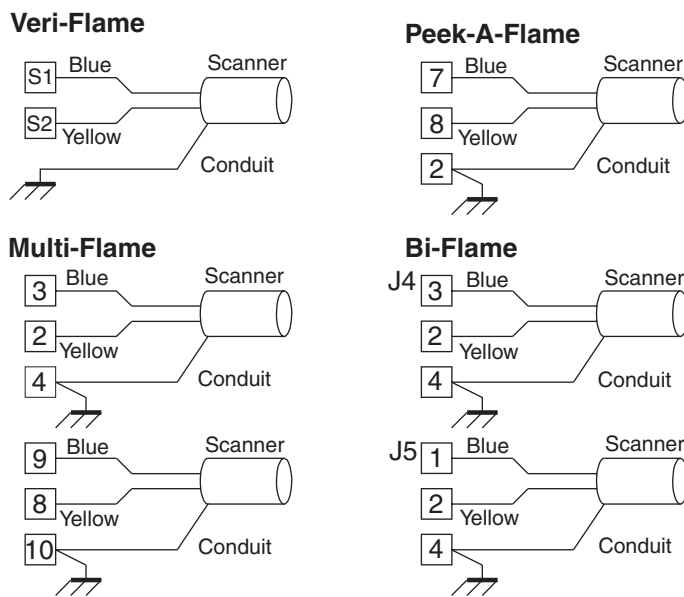
Figure 1 UV Scanner Wiring
